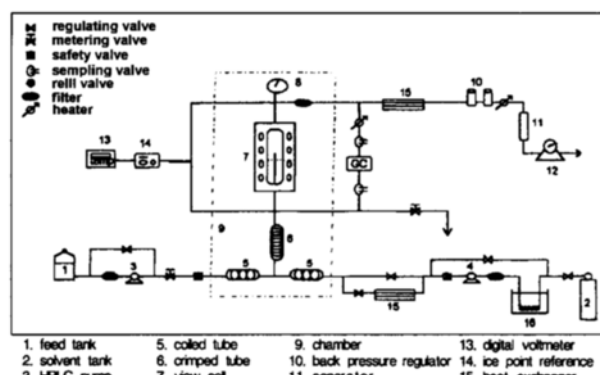
Fig. 1. Phase equilibrium apparatus.
